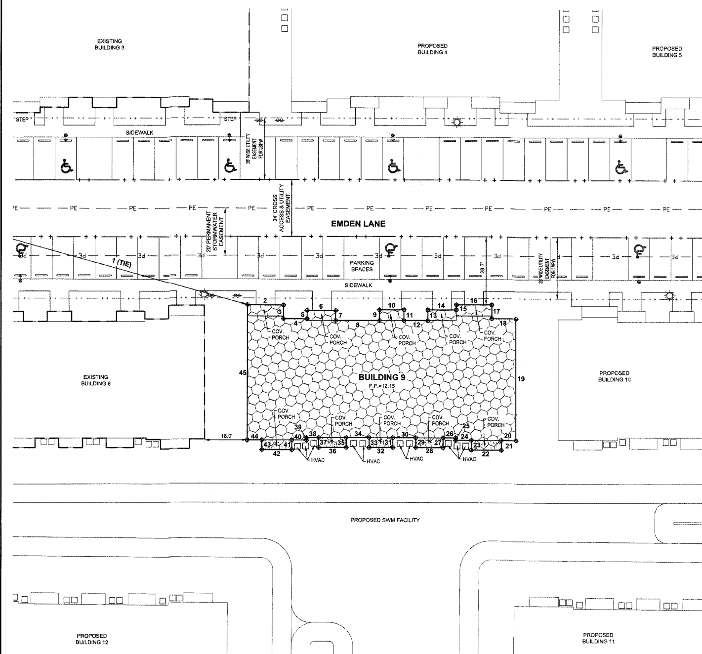
BUILDING 9 DETAIL SCALE: 1"=20'
