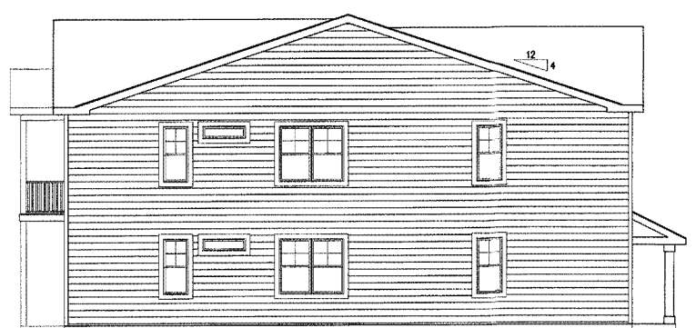
L. SIDE ELEVATION, BLDG 9 SCALE: 1/8"=1'0"
