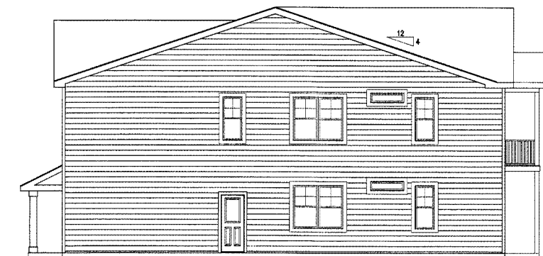
R. SIDE ELEVATION, BLDG 9 SCALE: 1/8"=1'0"
